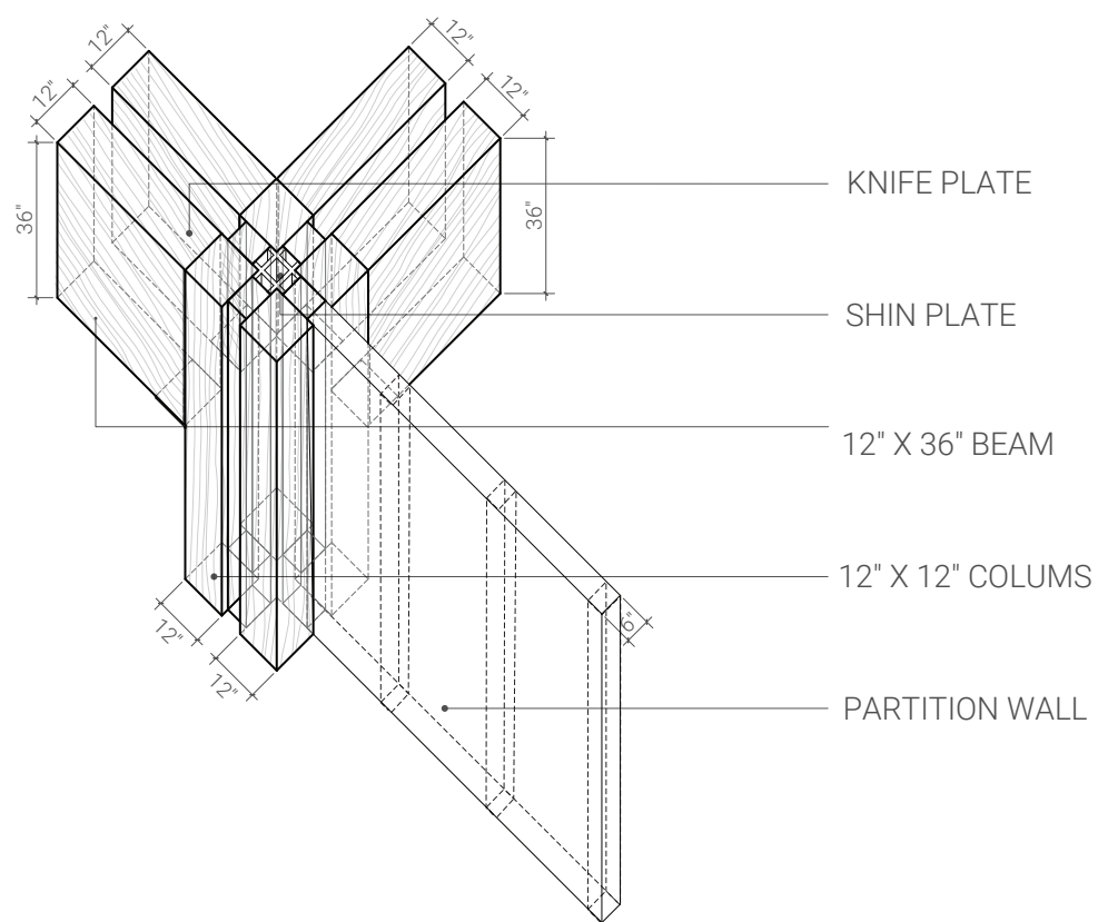
BEAM & PARTITION CONNECTION DETAIL SCALE: 1/4" = 1'-0"
