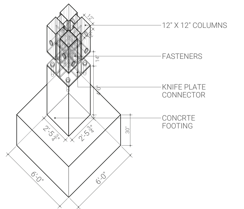
COLUMN AND FOOTING DETAIL SCALE: 1/4" = 1'-0"
