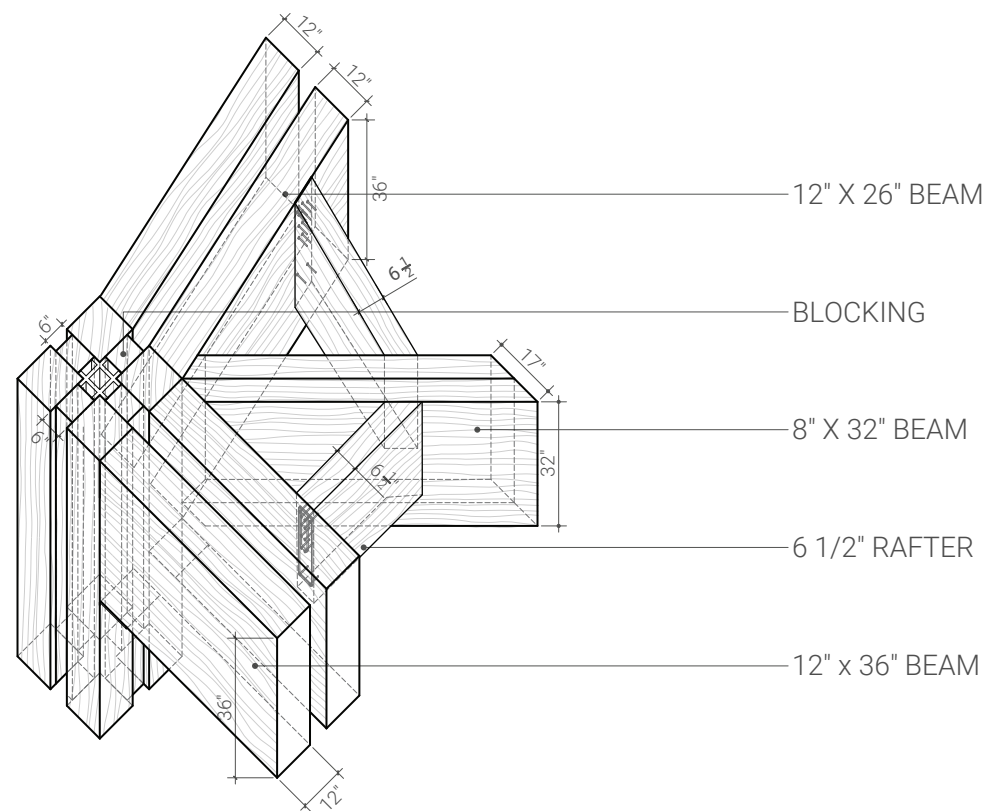
RAFTER & BEAM CONNECTION DETAIL SCALE: 1/4" = 1'-0"
